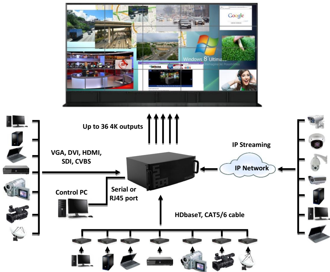
System Diagram
